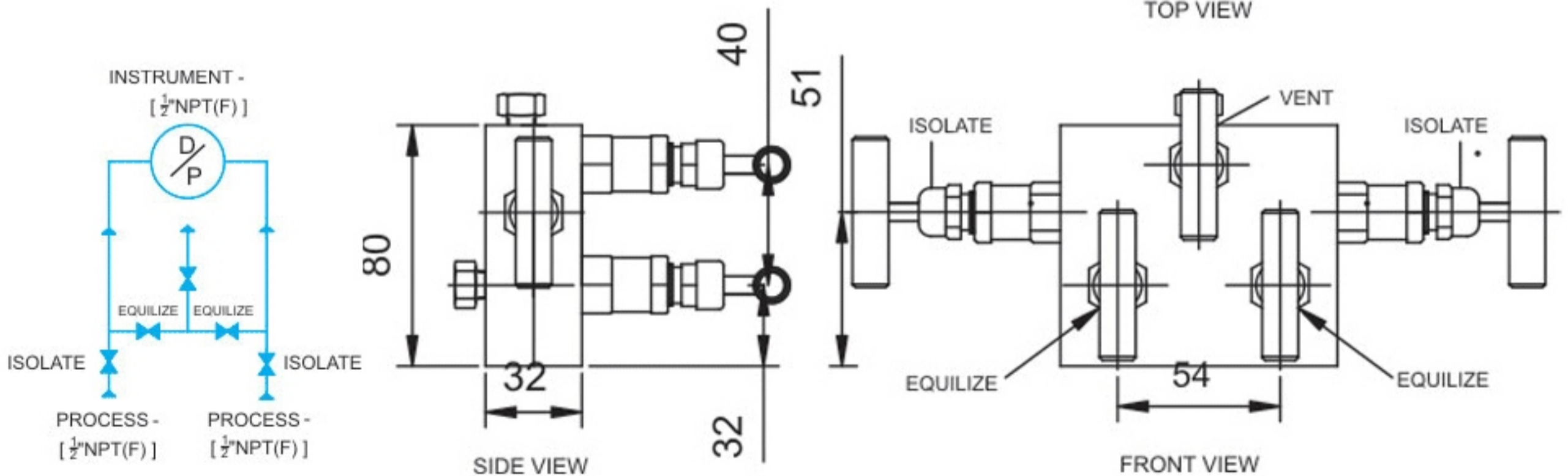
TOP VIEW
